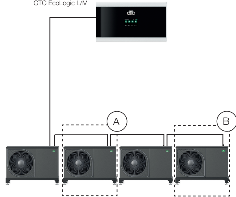
CTC EcoLogic L/M
