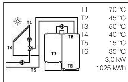
System 4 EcoHeat+Buffertank
