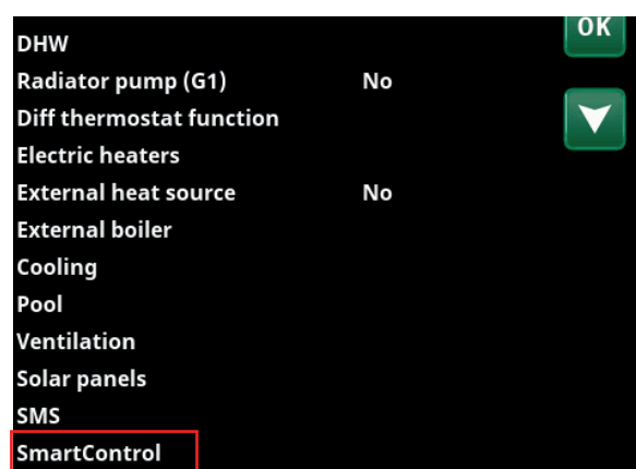
Menu "Installer/Define".
