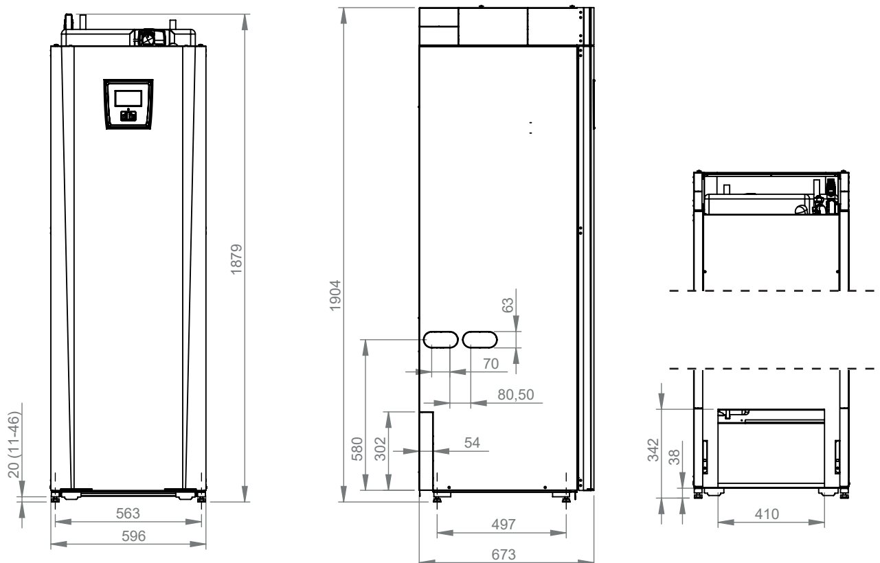
Model wysoki - CTC EcoZenit i255H
