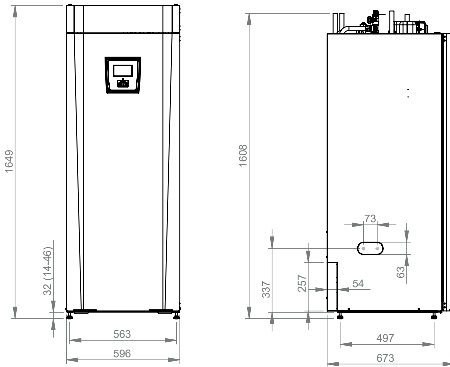
Model niski - CTC EcoZenit i255L
